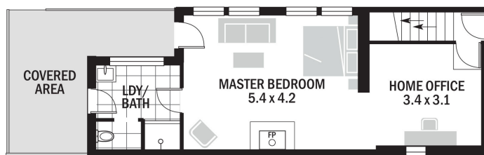
Lower Level Floor Plan
