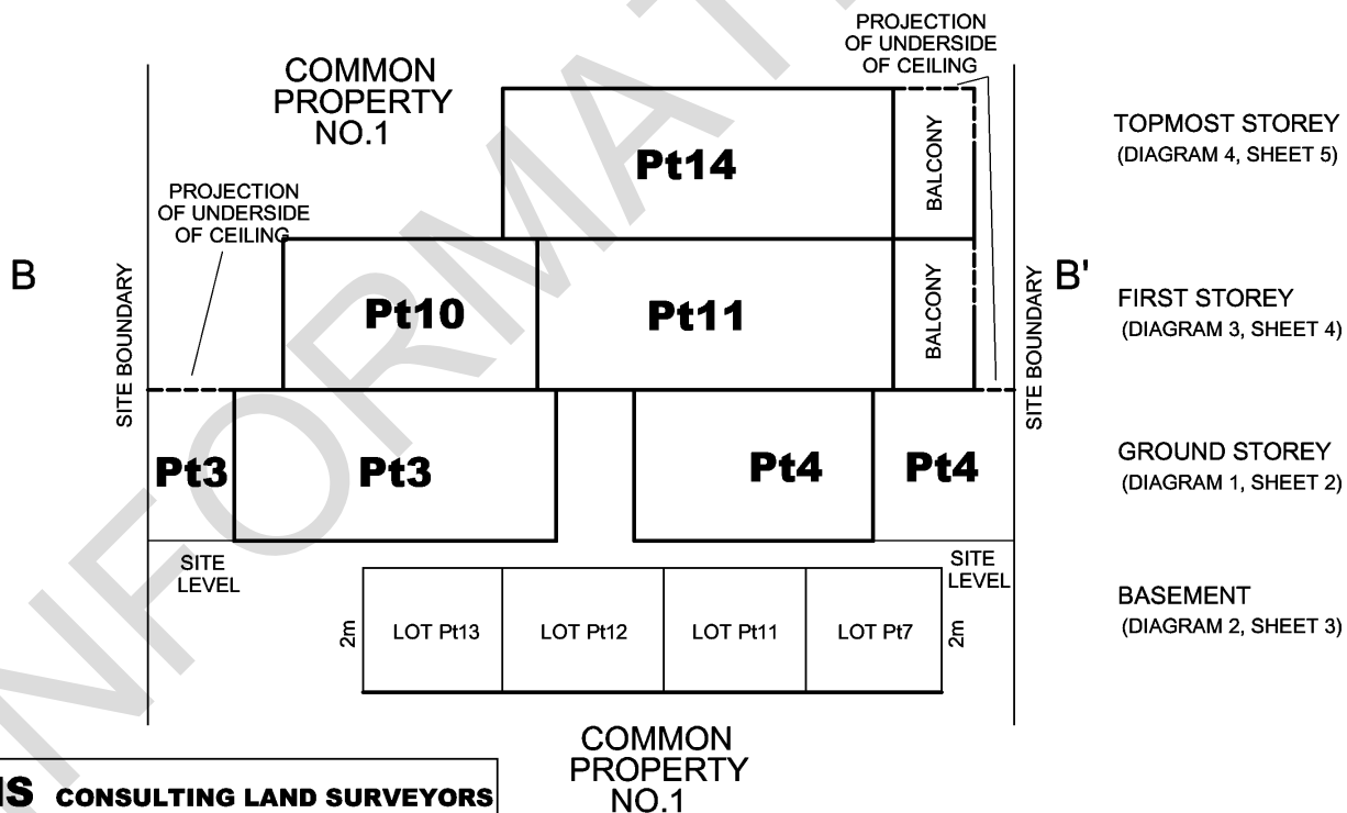
DIAGRAM 9 SECTION B - B'
