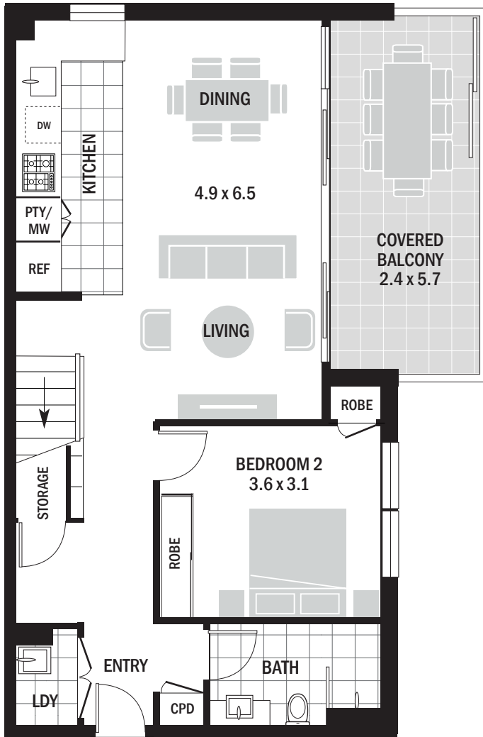
Entry Level Floor Plan
