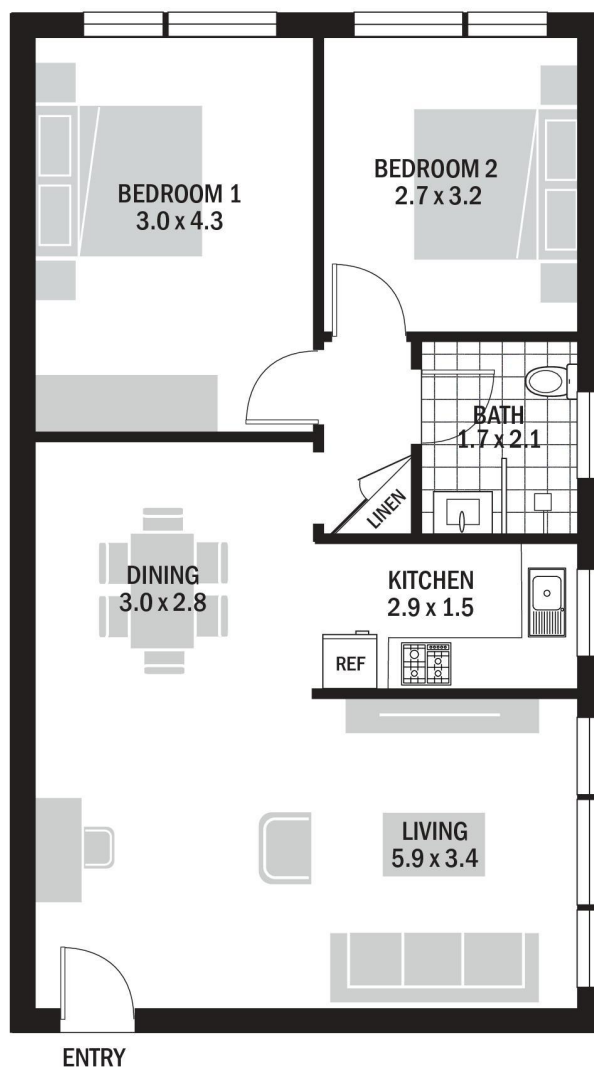
Apartment Floor Plan
