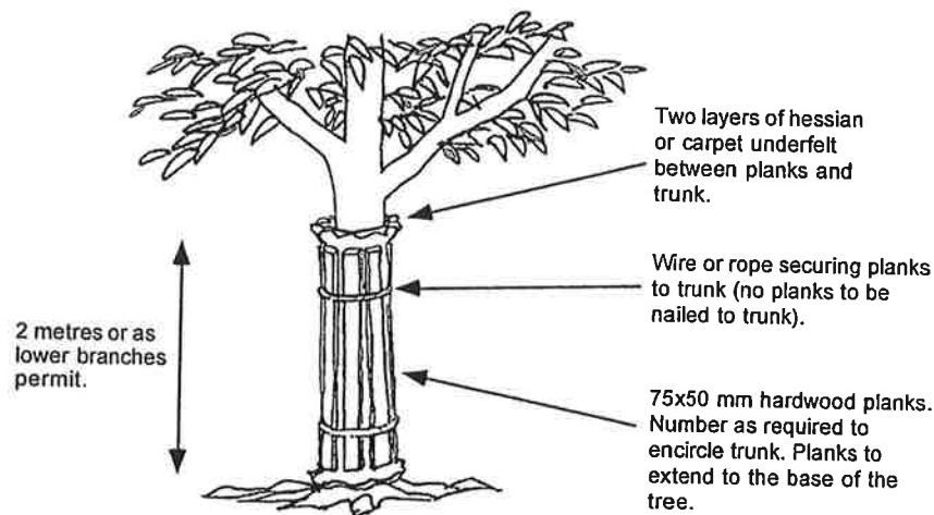
Diagram 1: Method of installing trunk protection.
