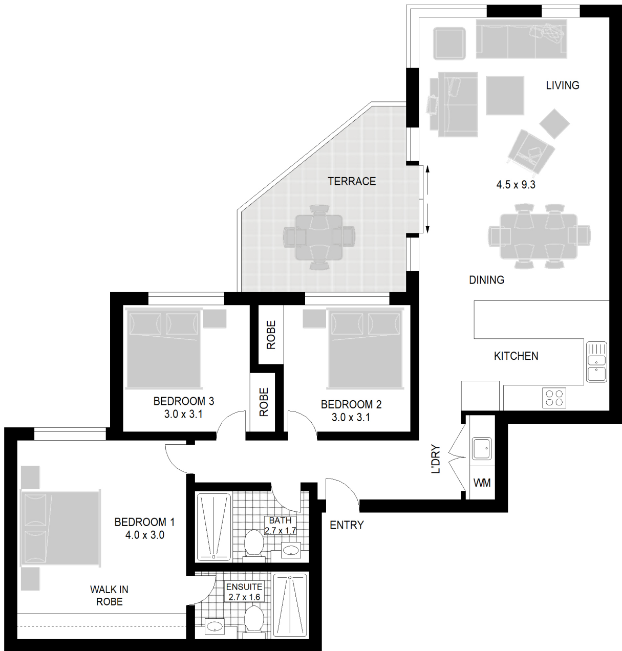
FIRST FLOOR
