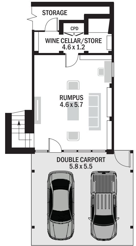
Lower Ground Floor Plan
